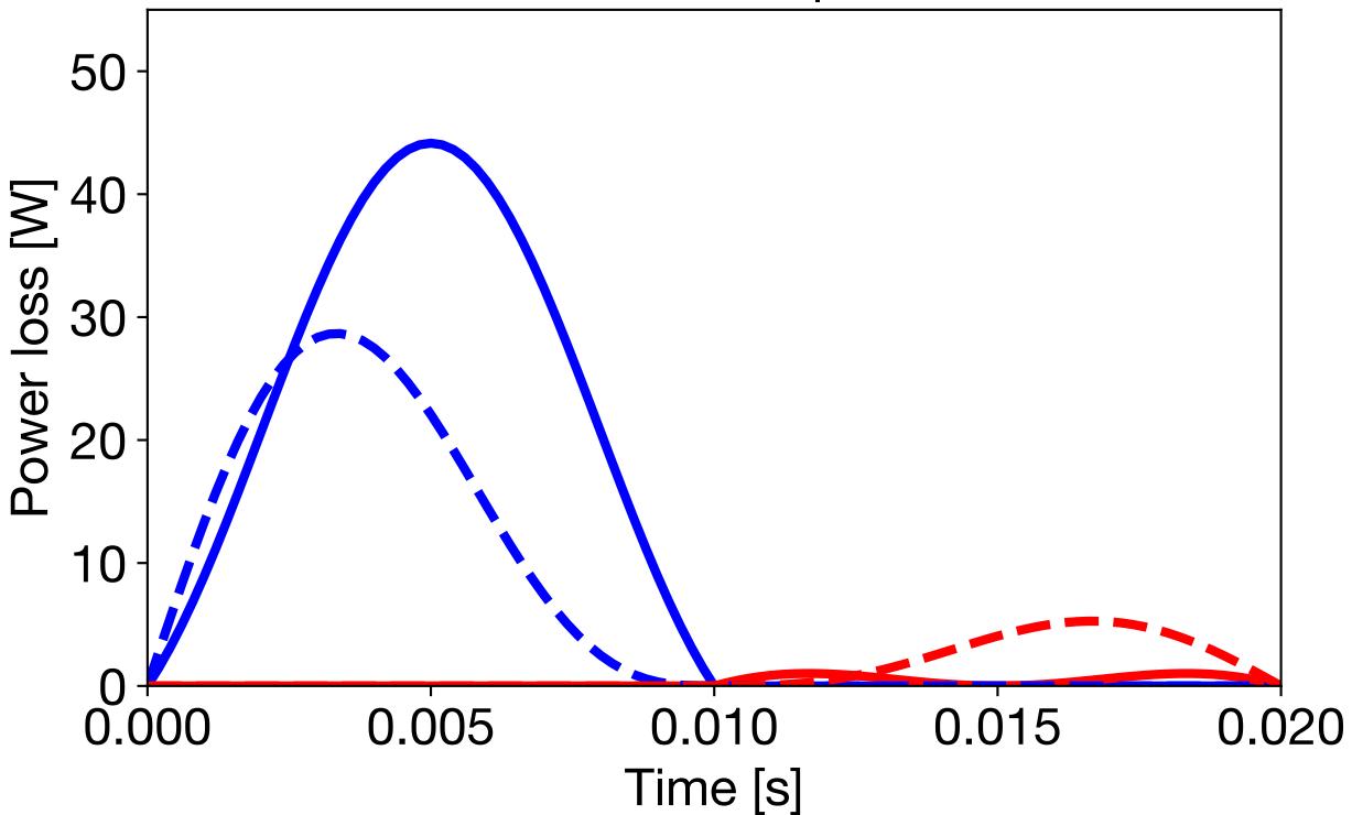
Total IGBT and diode power losses
